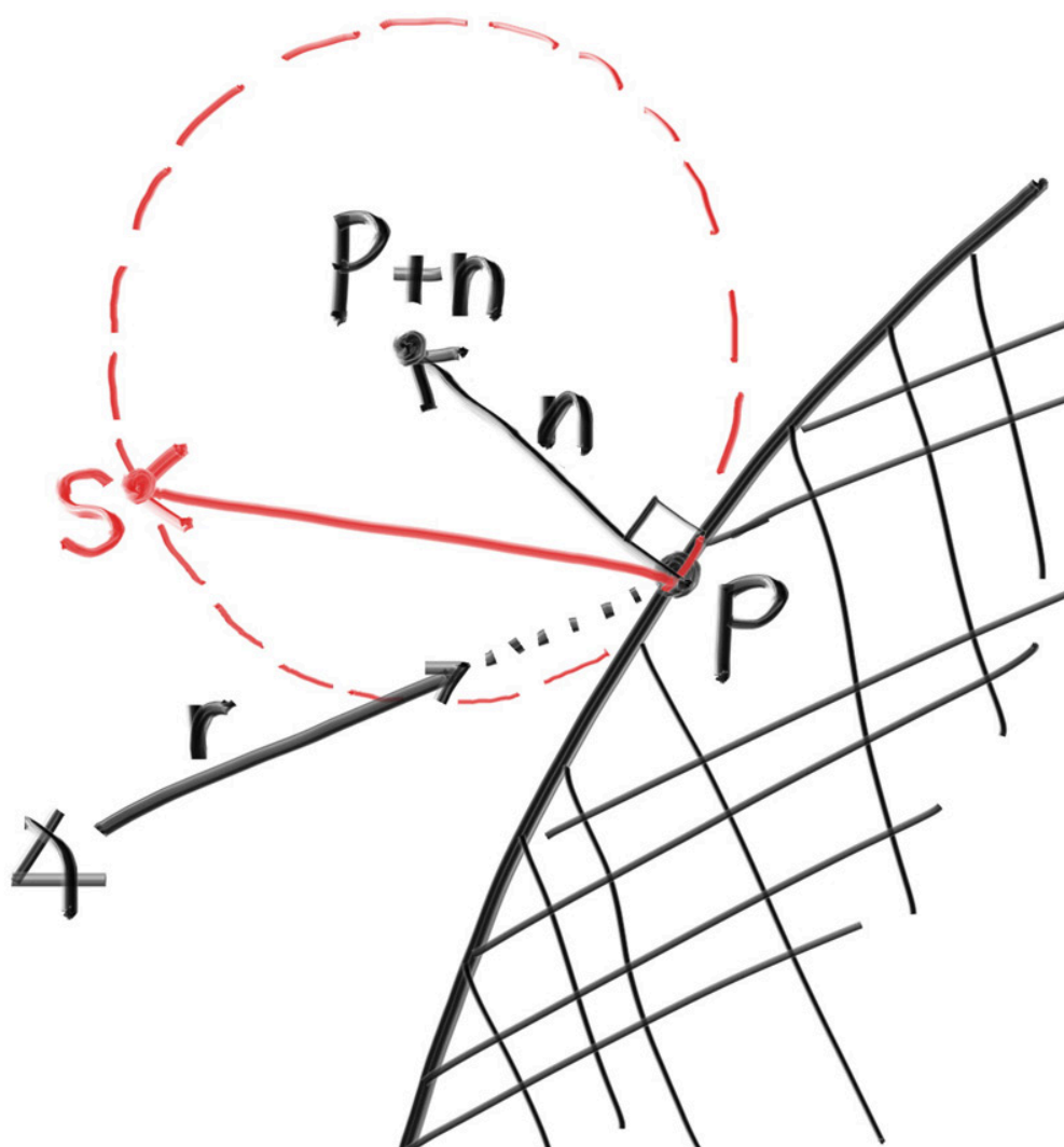
Figure 14: Randomly generating a vector according to Lambertian distribution
